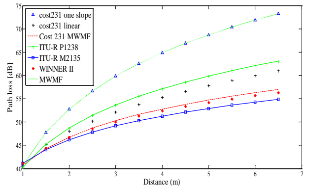
Fig. 4 Path loss for scenario A
